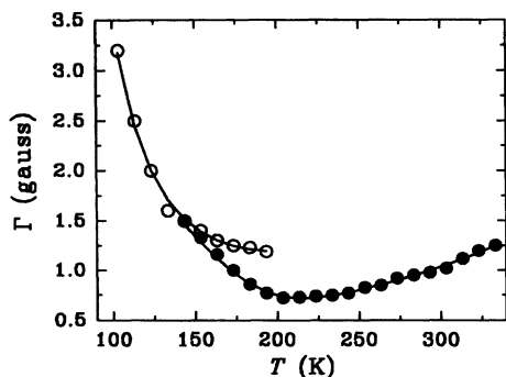
FIG. 3. Temperature dependence of the linewidth of the m_i = +1/2 (see Fig. 1) EPR transitions for \text{Sc}_3@C_{82} in frozen (filled circles) and fluid (open circles) decaline. The solid lines are fits of the dynamical model discussed in the text to the data.
