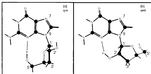
Figure 2. Syn (a) and anti (b) conformations of 3'-deoxyGs. Gs has -\text{OH} in both 2' and 3' positions. 2'-deoxyGs has -\text{OH} only in the 3' position. Dotted lines indicate hydrogen bonding.
